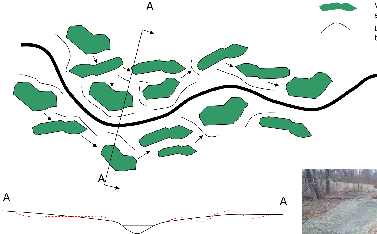
Project Headwaters Phase I Implementation: Site 1 – College Settlement Camp Riparian Stormwater Wetlands Concept Design N.T.S.
